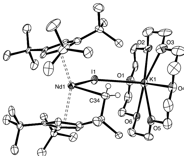
Figure 2. Molecular structure of the “tuck-in” complex [\text{Cp}^{\text{III}}\{\text{C}_5\text{H}_2\text{tBu}_2\text{C}(\text{CH}_3)_2(\text{CH}_2)_2\}\text{Nd}(\mu\text{-I})\text{K}([18]\text{crown-6})] ( 4 ). Thermal ellipsoids are set at 50% probability and hydrogen atoms are omitted for clarity (except for the methylene group). Hexane molecules present in the lattice are not represented.
